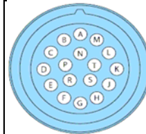
17 Pin - MS style mating-half & Pin information
