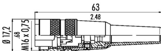
Amphenol / Binder style mating-half available in 5 Pin, 8 Pin & 12 Pin
