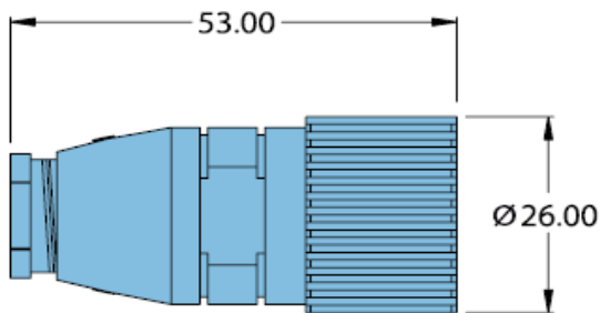
12 Pin & 16 Pin - Contact style mating-half & Pin information
