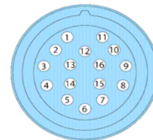
12 Pin & 16 Pin - Contact style mating-half & Pin information
