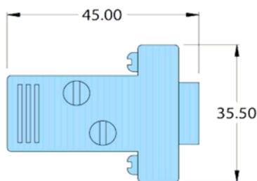
9 Pin D-Type style mating-half & Pin information
