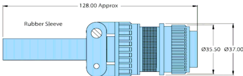
17 Pin - MS style mating-half & Pin information
