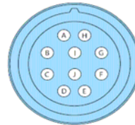
10 Pin - MS style mating-half & Pin information
