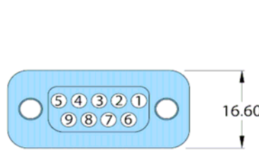
9 Pin D-Type style mating-half & Pin information
