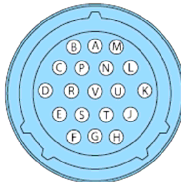
19 Pin - MS style mating-half & Pin information
