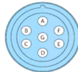
7 Pin - MS style mating-half & Pin information
