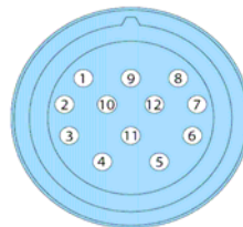
12 Pin & 16 Pin - Contact style mating-half & Pin information
